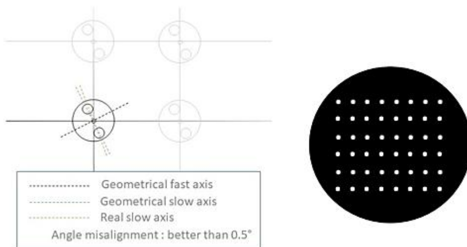
2D 光纤阵列 (SM, MM or PM)
