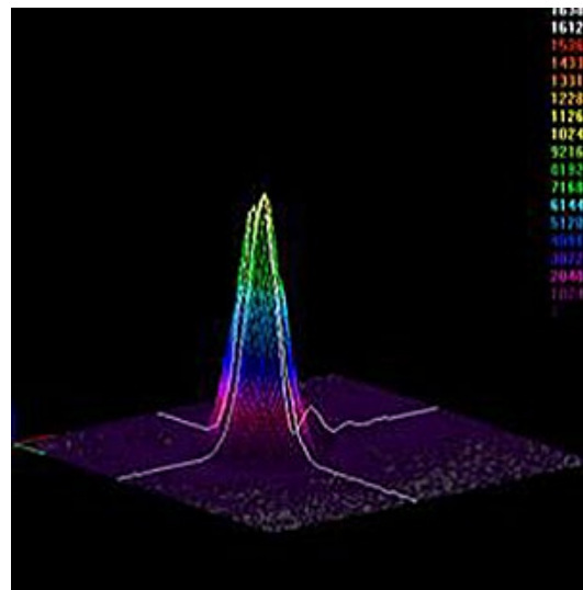
3-D Beam Profile at 1524.0 mm (60.0 in)
