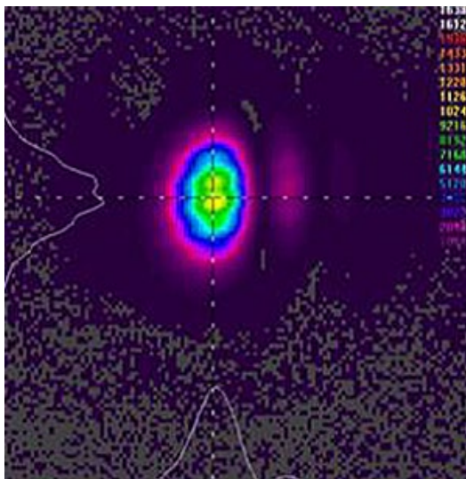
2-D Beam Profile at 1524.0 mm (60.0 in)
