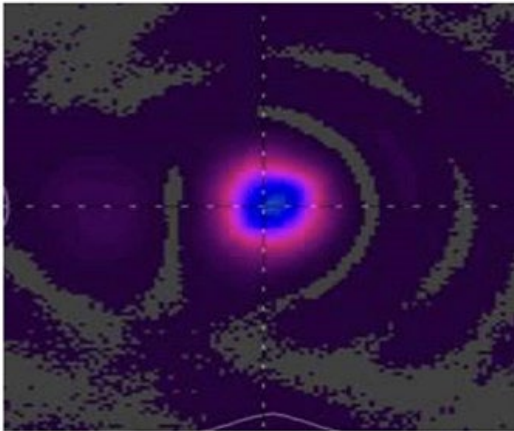
2-D Beam Profile at 1016.0 mm (40.0 in)
