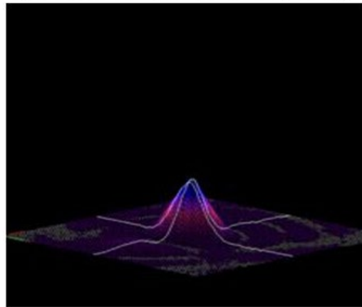
3-D Beam Profile at 1016.0 mm (40.0 in)
