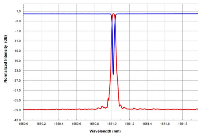
Transmission spectrum(透射光谱)
