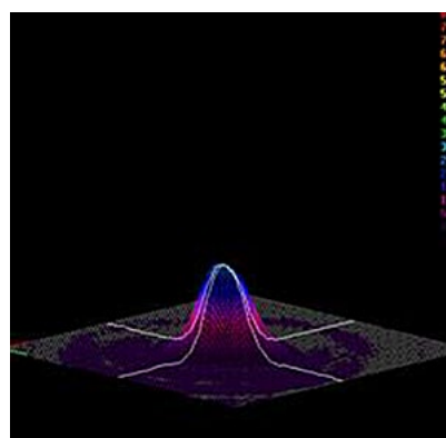
3-D Beam Profile at 762.0 mm (30.0 in)
